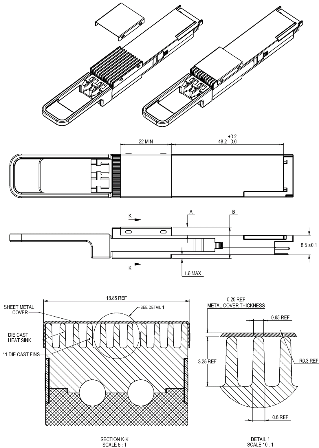
Figure 39 Type 2A and 2B examples of die Cast Heat Sink Example
