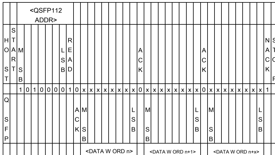
Figure 34 Sequential address read starting at QSFP112 current address
