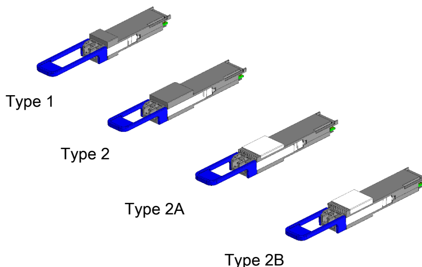
Figure 29 QSFP112 Module variants: Type 1; Type 2; Type 2A; and Type 2B
