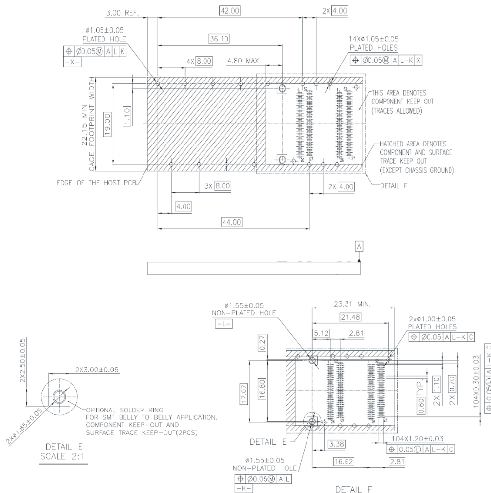
Figure 17 QSFP112 2X1 SMT Connector and cage PCB layout
