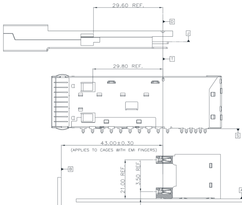
Figure 11 QSFP112 2X1 SMT Connector/Cage/Module Datum
