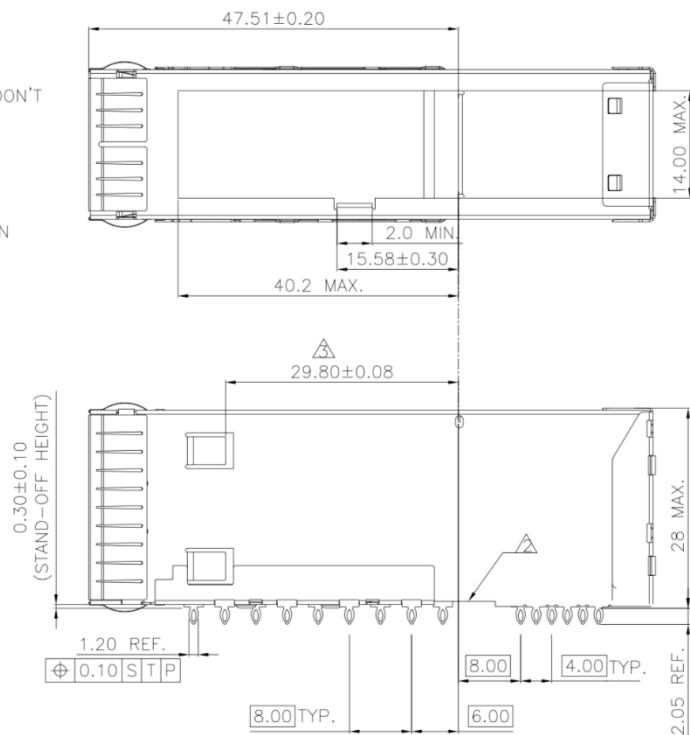
Figure 24 QSFP112 2X1 Cage
