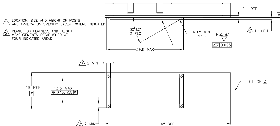
Figure 25 QSFP112 Heatsink
