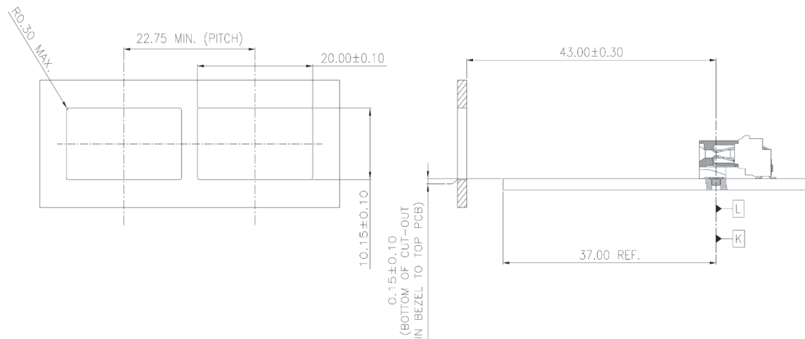
Figure 18 QSFP112 1X1 SMT Bezel opening
