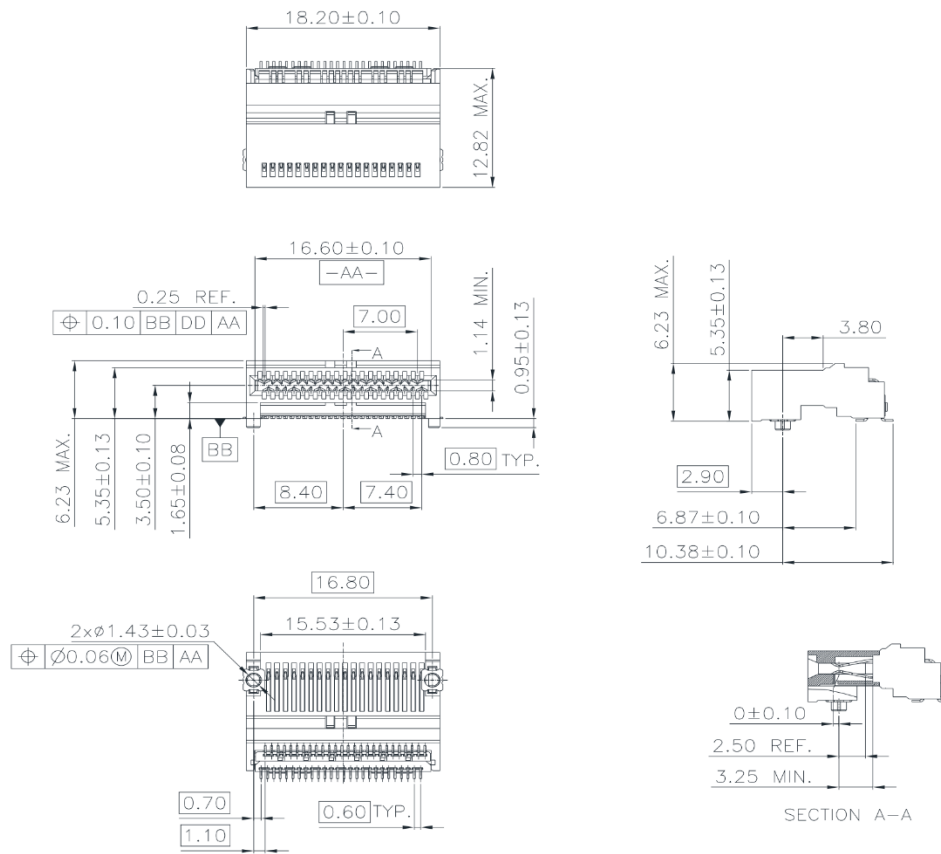
Figure 21 QSFP112 1X1 SMT Connector
