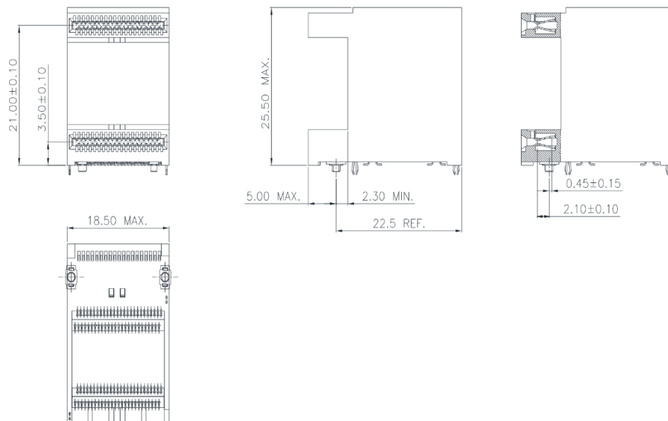
Figure 22 QSFP112 2X1 SMT Connector
