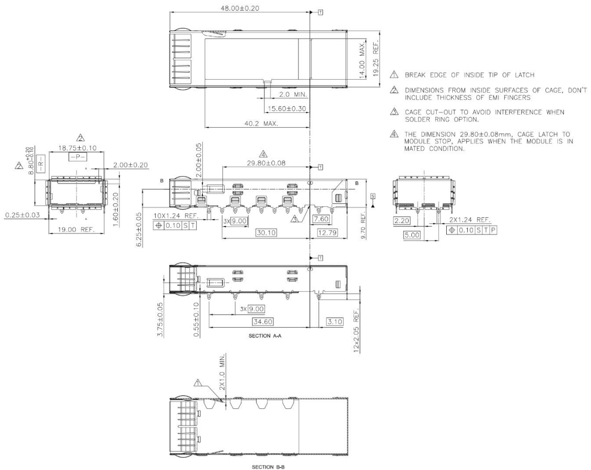
Figure 23 QSFP112 1x1 Cage
