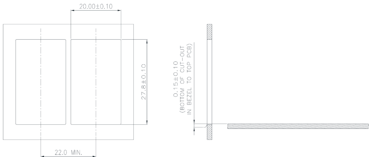
Figure 19 QSFP112 2X1 SMT Bezel opening
