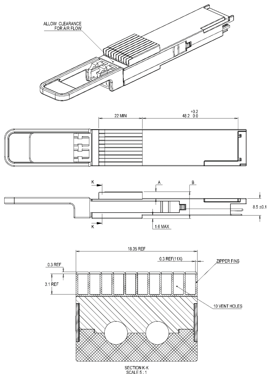
Figure 40 Type 2A and 2B examples of zipper Fin Heat Sink Example
