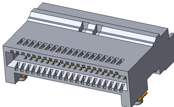
Figure 20 QSFP112 Module electrical connector illustration
