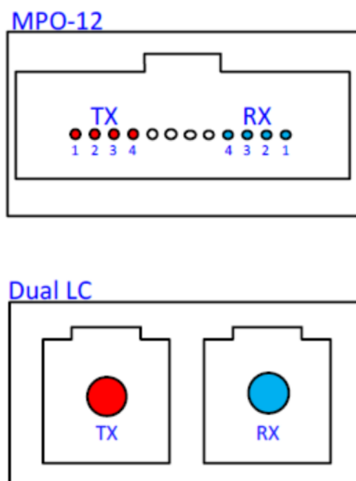
Figure 26 Optical media dependent interface port assignments
