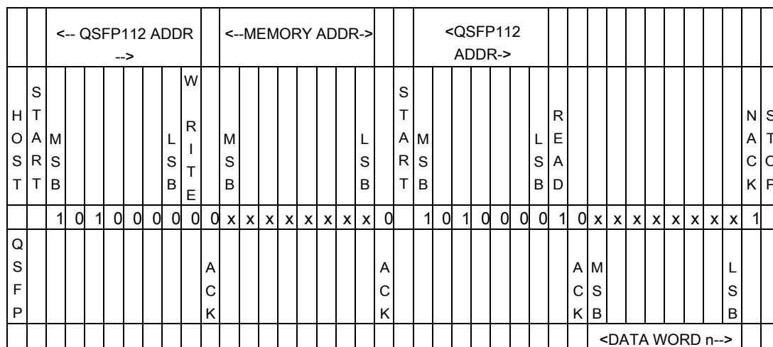
Figure 33 QSFP112 Random read
