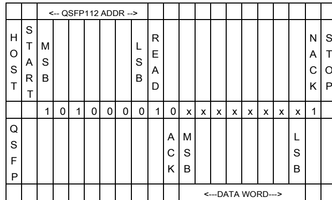
Figure 32 QSFP112 Current address read operation
