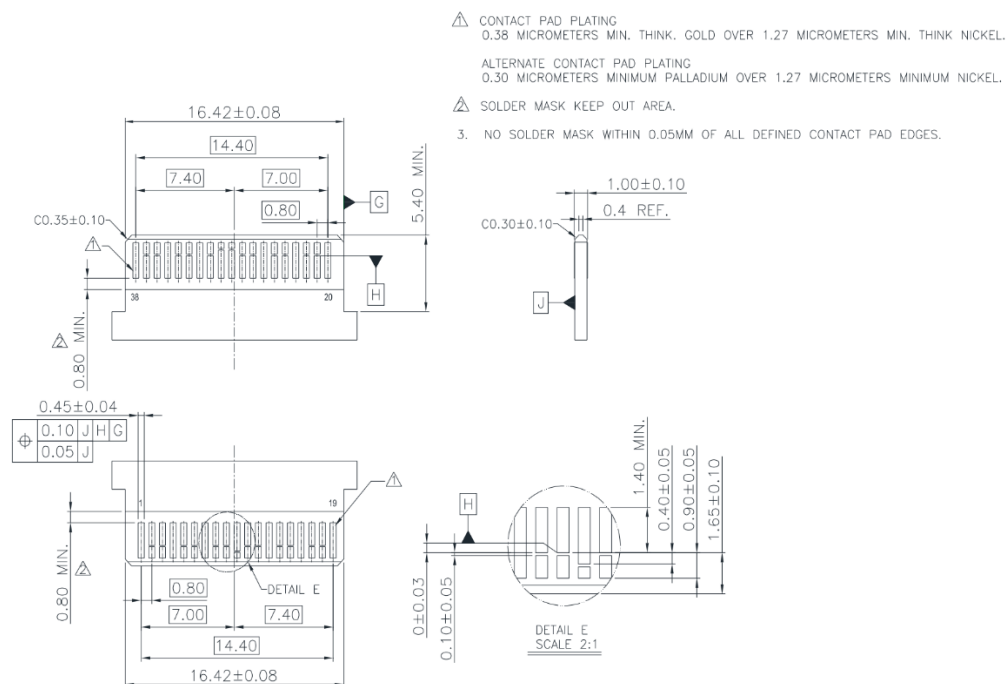
Figure 14 QSFP112 Improved paddle card dimensions
