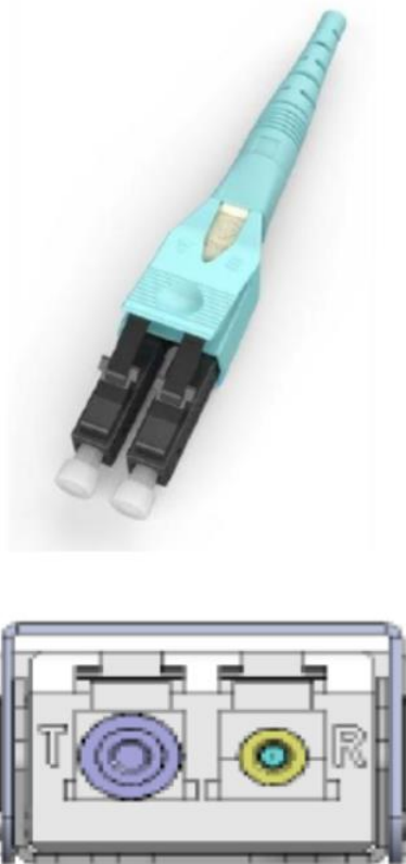
Figure 28 Dual LC optical patchcord and module receptacle
