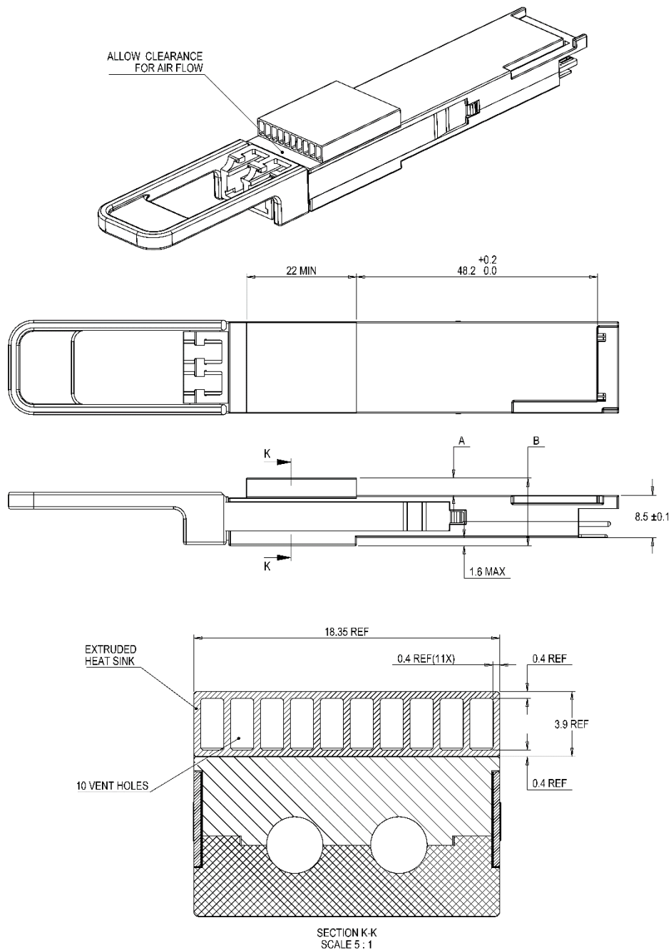
Figure 38 Type 2A and 2B examples of extruded Heat Sink Example
