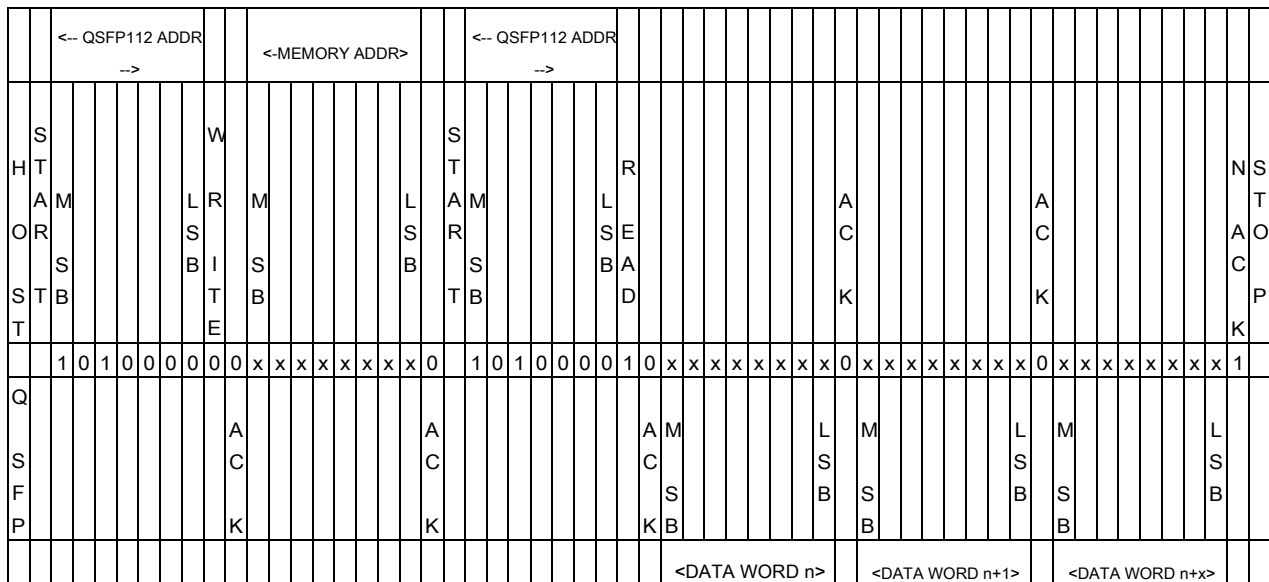
Figure 35 Sequential address read starting with random QSFP112 read
