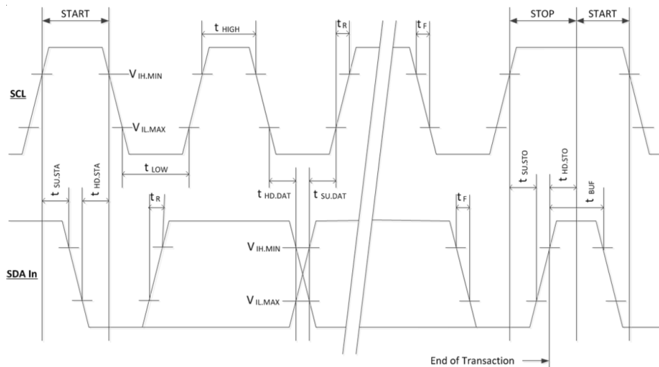
Figure 30 TWI Timing diagram
