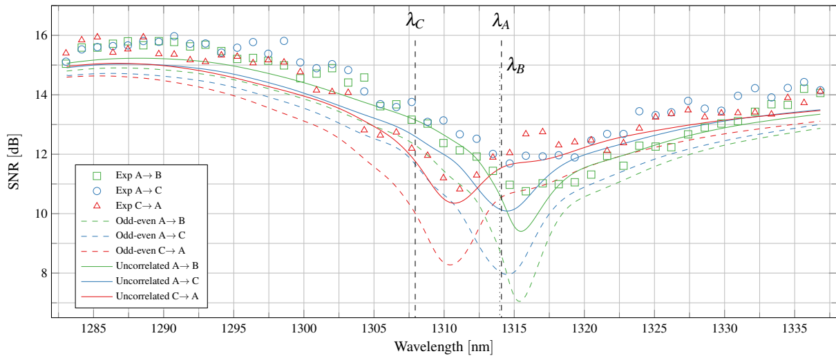
Fig. 4: After two span transmission the SNR of the central channel at a fixed per channel launch power of +6 dBm for different span orders. Coloured lines showing the SNR from simulations, dashed for odd-even and solid for uncorrelated channels. Vertical dashed lines showing the zero dispersion wavelengths of Span A, B and C
