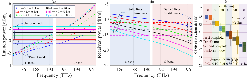
Fig. 1. (a) Launch and (b) received power profiles for the pre-tilt and uniform modes for span lengths from 50 km to 100 km. (c) GSNR boxplots of all channels for span lengths from 50 km to 100 km.
