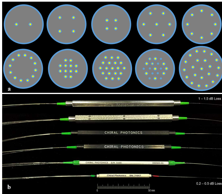
Fig. 1. (a) Various types of MCFs which have been addressed by the VCF-fanouts. (b) Evolution of MCF fanout technology over last decade 2013 - 2023.
