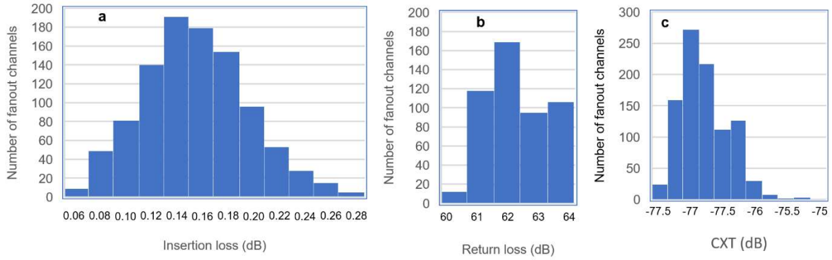
Fig. 2. Distributions of C-band average insertion loss (a), return loss (b), and counter-propagating crosstalk (c) for last 500 fabricated 2-core fanouts, fusion spliced to 2-core MCF.
