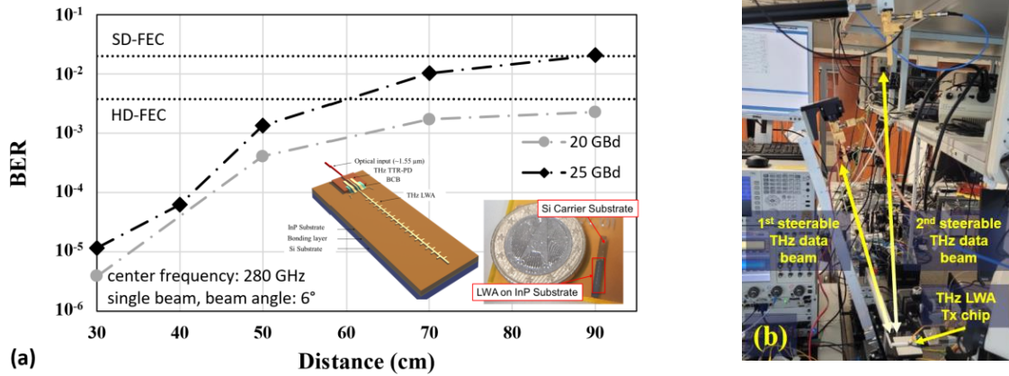
Fig. 2. Measured BER vs. distance for single THz beam. Insets show schematic and photo of fabricated photonic assisted LWA (a). Multi-beam operation with two THz Rx at 6° and 20° with distances of 70 cm and 50 cm (b).
