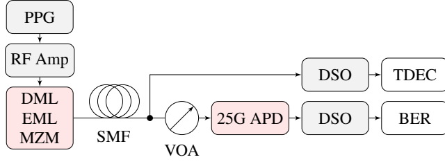
Fig. 1: Experimental setup
