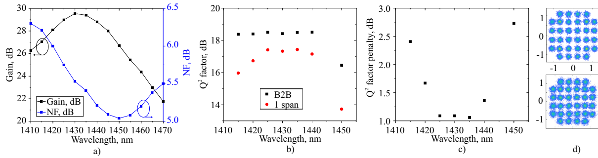
Fig. 2. a) Spectral dependence of the gain and NF of the receive BDFA; b) Spectral dependence of Q^2 factors for B2B and single span measurements for SP-QPSK signal; c) Spectral dependence of the Q^2 penalties for SP-QPSK signal; d) SP-32-QAM constellations for B2B measurement (top) and single span transmission measurement (bottom).
