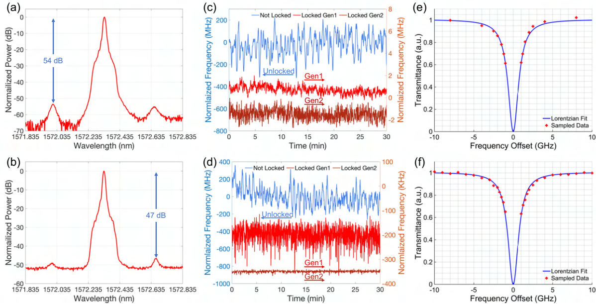
Fig. 3. (a) First generation locked leader laser spectrum. (b) Second generation locked leader laser spectrum. (c) Comparison of leader laser stabilization. (d) Comparison of follower laser stabilization. (e) First generation CW sampling of CO 2 with Lorentzian fit. (f) Second generation CW sampling of CO 2 with Lorentzian fit.
