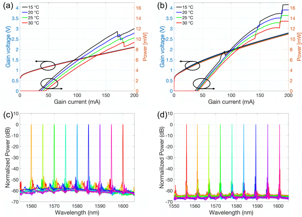
Fig. 2. (a) First generation light-current-voltage curve measured at the SOA. (b) Second generation light-current-voltage curve measured at the SOA. (c) First generation laser tuning. (d) Second generation laser tuning.
