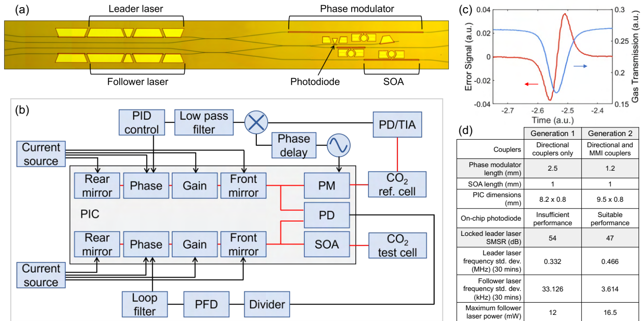
Fig. 1. (a) Microscope image of fabricated first generation PIC. (b) Test setup used to characterize PIC. PID = proportional-integral-derivative. PD/TIA = photodiode/transimpedance amplifier. PM = phase modulator. PFD = phase frequency detector. (c) Absorption and error signal at the reference gas cell detector. (d) Table comparing the layout and performance of first and second generations.
