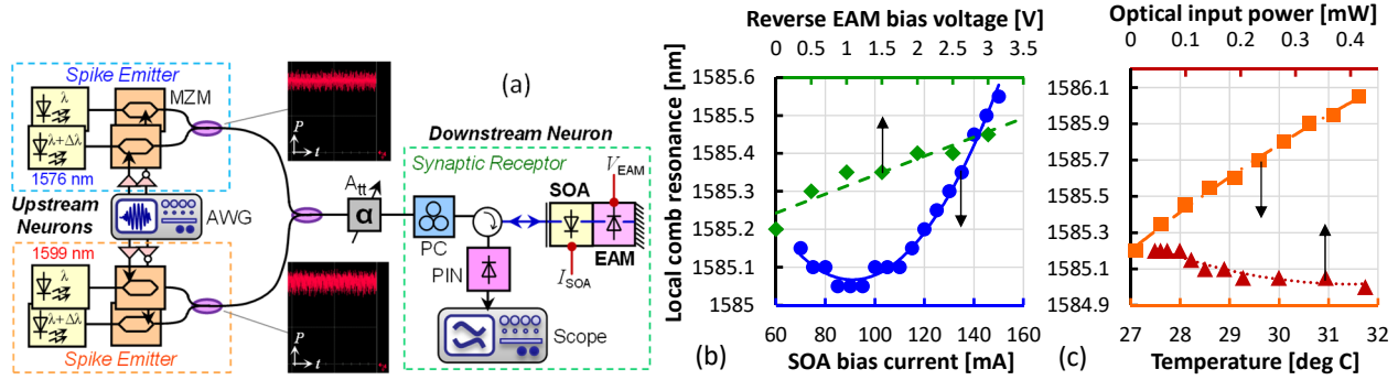
Fig. 2. (a) Experimental setup. (b) SOA+EAM transfer function shift with SOA and EAM bias, and (c) temperature and optical input power.
