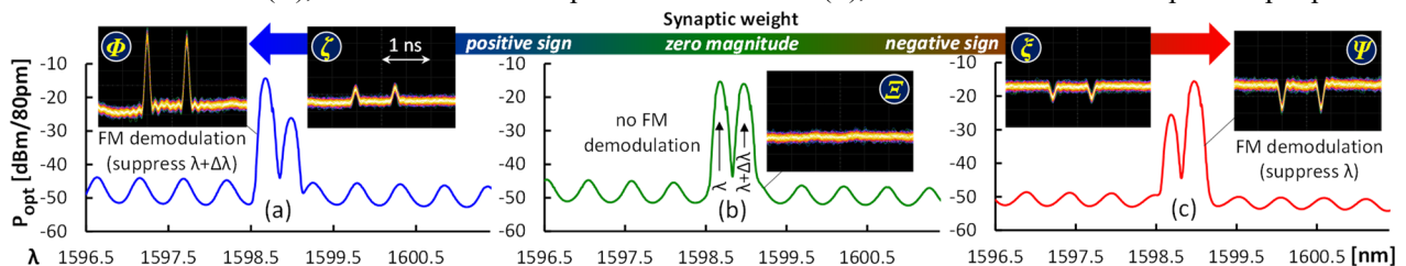
Fig. 3. Signal spectra and received spike train for the weighing process with SOA+EAM: (a) positive sign, (b) zero magnitude, (c) negative sign.
