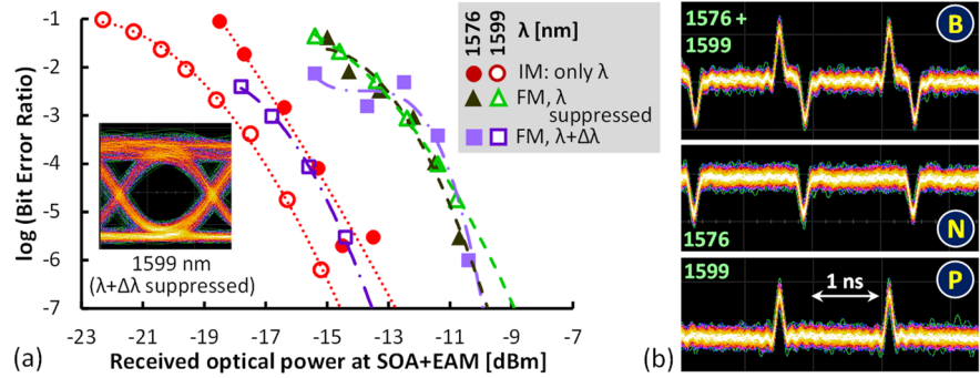
Fig. 4. (a) BER performance. (b) Simultaneous MAC for spike trains at 1576 and 1599 nm.
