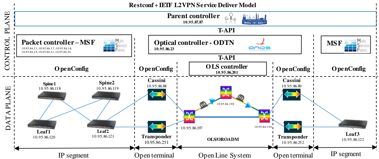
Fig. 3. Experimental setup
