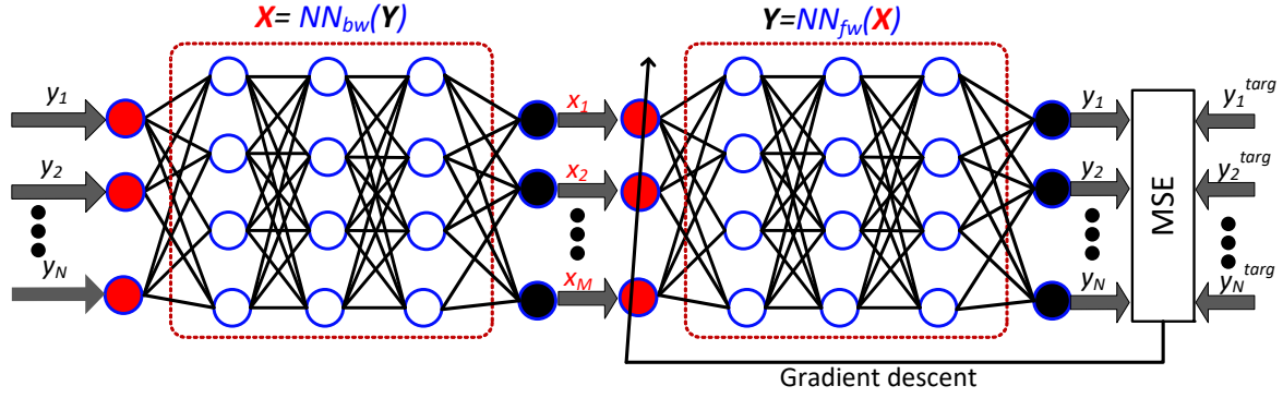
Fig. 1. Illustration of the machine learning based approach for the inverse system design [4].
