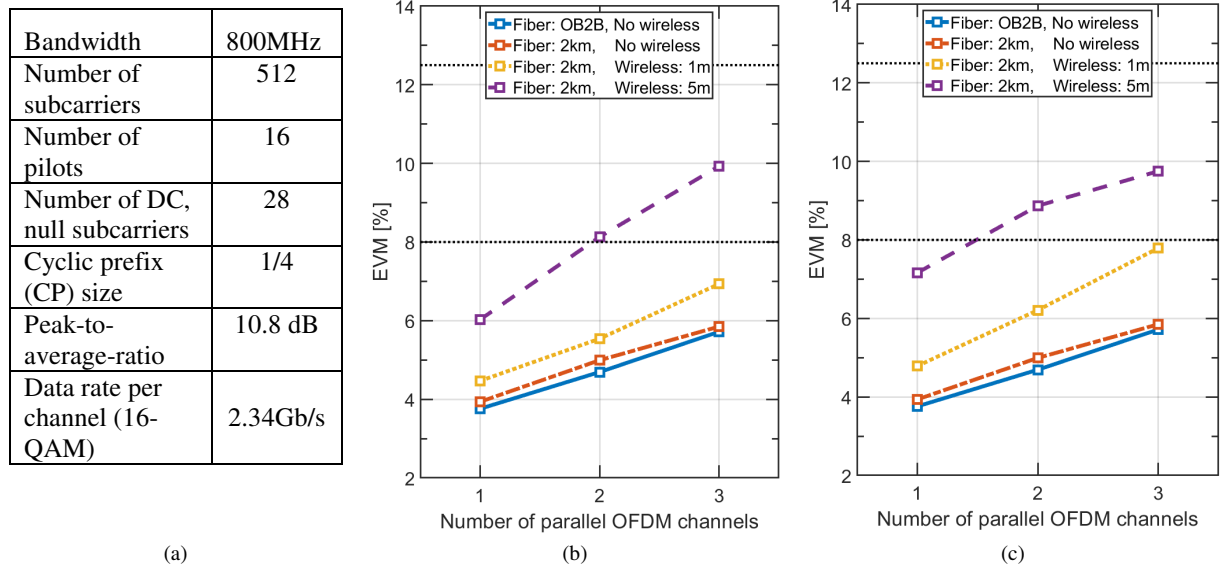
Fig. 4: (a) OFDM signal parameters. (b) Measured EVM in RFoF-wireless downlink. (c) Measured EVM in RFoF-wireless uplink.
