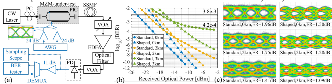
Fig. 3: (a) experimental setup: PC: polarization controller, VOA: variable optical attenuator; (b) BER curves for the standard and shaped MZM for 56 Gb/s over 0, 2 and 3 km as a function of power incident on the EDFA; (c) eye diagrams of the standard and shaped MZM for 56 Gb/s.
