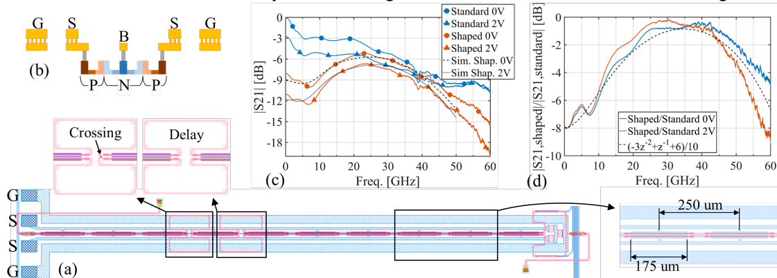
Fig. 2: (a) Layout of the MZM with shaping, insets of the crossing, delay and segments; (b) cross section of the transmission line at a segment; (c) simulated and measured electro-optic transfer function (d) measured effect of the transfer function shaping compared to the theoretical shape.
