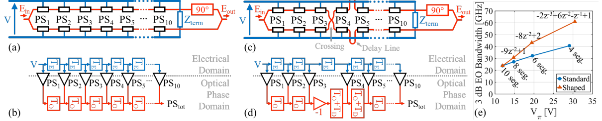
Fig. 1: (a) Standard 10-segment periodically loaded MZM; (b) equivalent block diagram of (a); (c) 10 segment periodically loaded MZM with transfer function shaping (d); equivalent block diagram of (c); (e): Simulation of standard MZM with 4, 6, 8 or 10 segments vs. various configurations of a shaped MZM with 10 segments. Note: the simulations accuracy decreases above 40 GHz.
