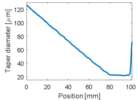
Fig 2. Taper profile measurement results.
