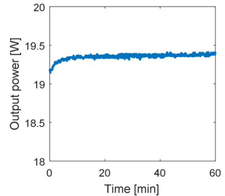
Fig. 6. Stability of the side-coupler over time
