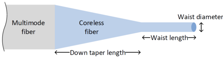
Fig. 1. Schematic of a half-taper.
