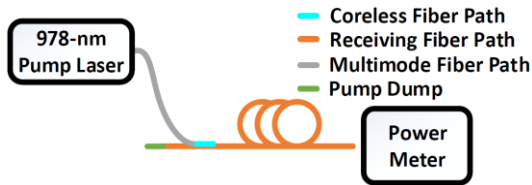
Fig. 3. Setup used for the characterization of the couplers.
