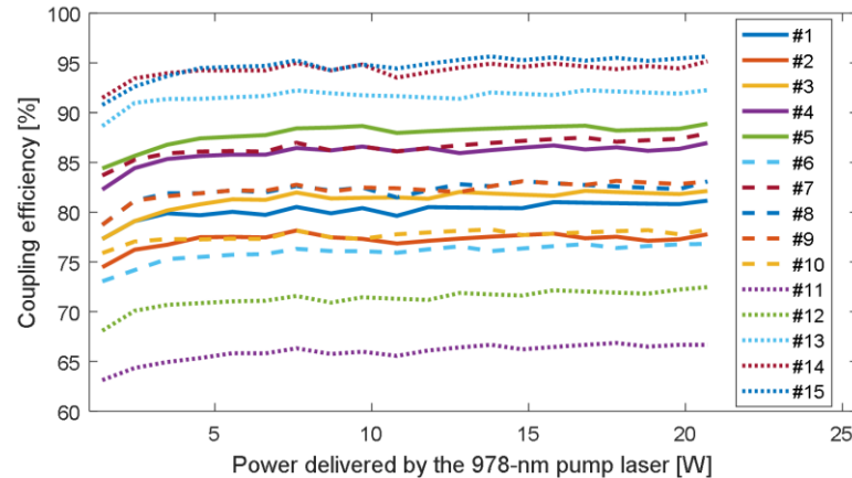
Fig. 5. Coupling efficiency as a function of power delivered by the 978 nm pump laser for all of the experiments.
