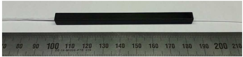
Fig 4. Packaging of the combiner/fan-in spliced to the 12c-EYDF
