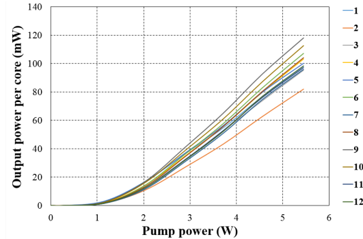
Fig. 8. Output power versus pump power for each
