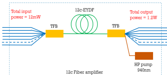
Fig. 5. Amplifier architecture
