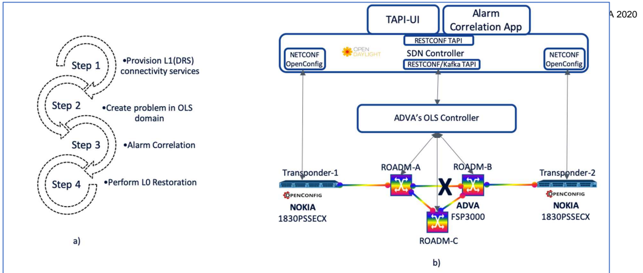
Figure 3: a) Alarm correlation demonstration scenario; b) Telefonica Lab testbed
