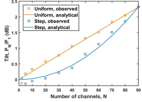
Fig. 2: Observed and analytical values of Raman tilt in case of uniform and step loading.
