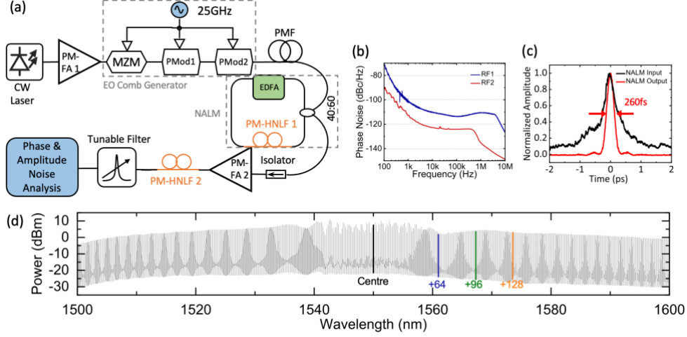
Fig. 1: (a) Experimental Setup. (b) RF phase noise of the 25-GHz signals: RF1 (blue) and RF2 (red). (c) Autocorrelator measurement for the pulses before (black) and after (red) the NALM, (d) Spectrum of the comb output (0.02 nm resolution).
