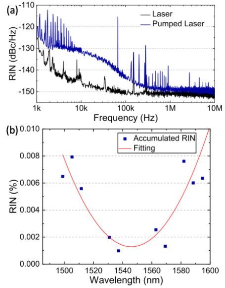
Fig. 4: RIN measurement for (a) laser (black) and pumped laser (blue). (b) Integrated RIN (blue square) and quadratic fitting (red curve) of the parametric comb.
