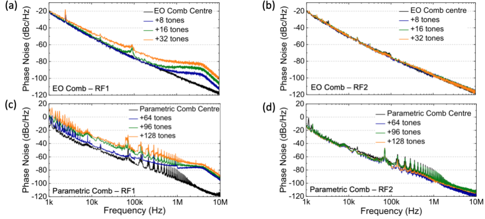
Fig. 3: Phase noise of EO comb using RF1 (a) and RF2 (b), and the broadened comb of +64 (blue), +96 (green) and +128 (orange) tone using RF1 (c) and RF2 (d), respectively.
