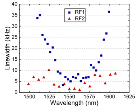
Fig. 2: Measured 100- \mu s linewidth for tone (with 400 GHz interval) of the parametric comb using two different RF generators: RF1 (blue square), RF2 (red triangle).
