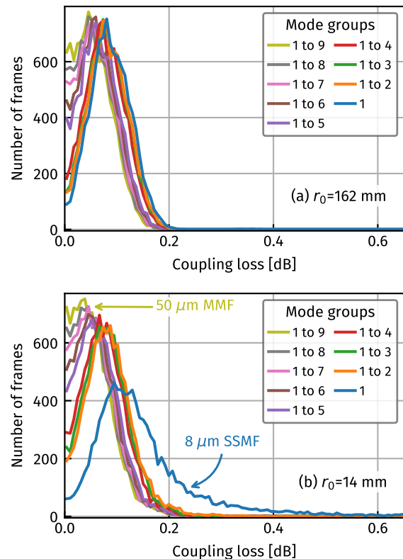
Fig. 3: Histogram of coupling loss over 10,000 frames for (a) r_0 = 162 mm and (b) r_0 = 14 mm
