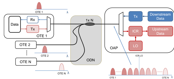
Fig. 1: P2MP access network system utilizing low latency FDMA sub-channels in the upstream.
