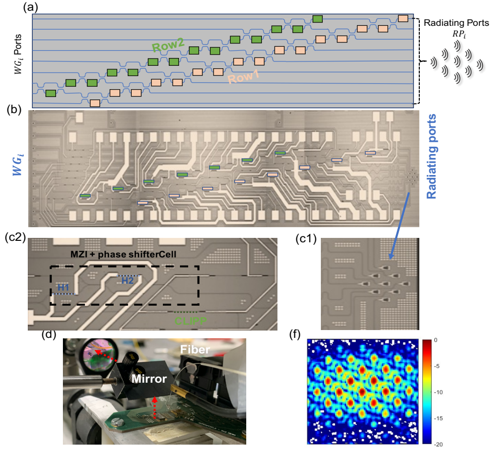
Fig. 1: (a) Schematic of the 9×2 diagonal mesh of MZIs with a pair of phase actuators in each stage (differentiated by colors for different rows of the mesh); (b) Microscopic picture of the fabricated silicon chip highlighting MZI elements of row 1 (yellow boxes) and 2 (green boxes). (c1) Detail of the 3×3 array of grating couplers used as radiation ports and (c2) of the MZI thermally tuneable beam coupler followed by a transparent detector (CLIPP). (d) Experimental setup showing the fiber coupling to the WG i ports of the mesh and turning mirror. (f) Collimated far field of the array captured with NIR camera when mesh is tuned to couple to a fiber collimator.
