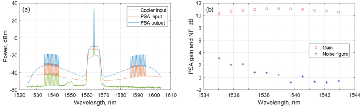
Fig. 4: (a) Optical spectra at the input and output of the copier and the PSA when amplifying WDM channels. (b) Gain and noise figure of each channel in the PSA.
