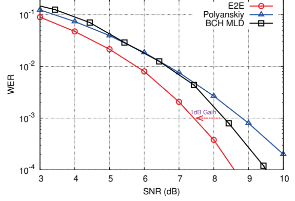
Fig. 2: AWGN performance for (4, 7) codeword.
